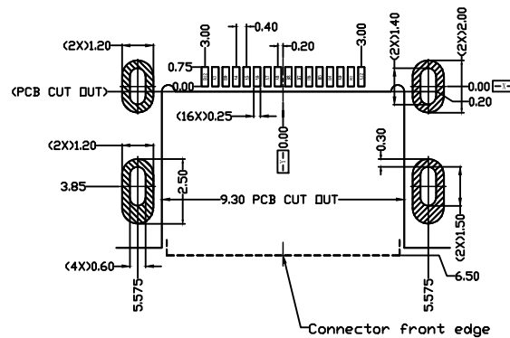
RECOMMENDED P.C.B LAYOUT TOP VIEW TOLERANCES ± 0.05MM
